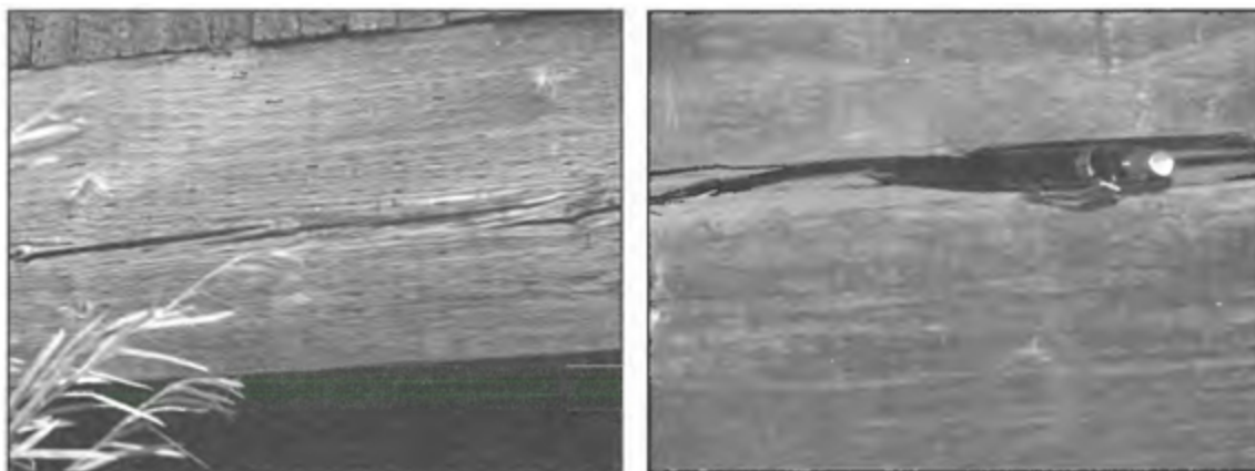
Figure B-2-2-in. Deep Check in Exterior Beam
