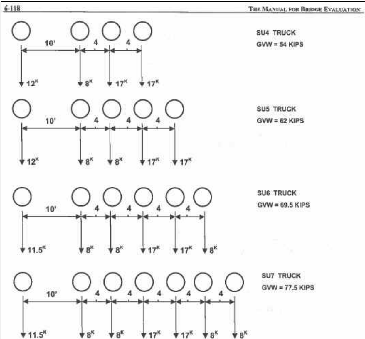
Figure 6B.9.2-2—Bridge Posting Loads for Single Unit Trucks that Meet Formula B
