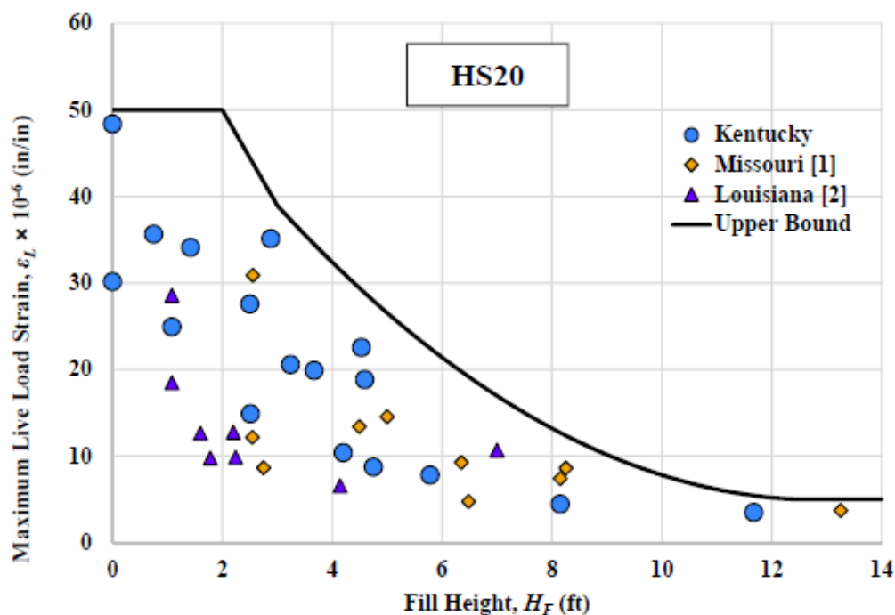
Fig. 1. Maximum Live Load Strain, \epsilon_L \times 10^{-6} (in/in), vs. Fill Height, H_F (ft) for field tested culverts, adjusted to the AASHTO HS20 design truck.
