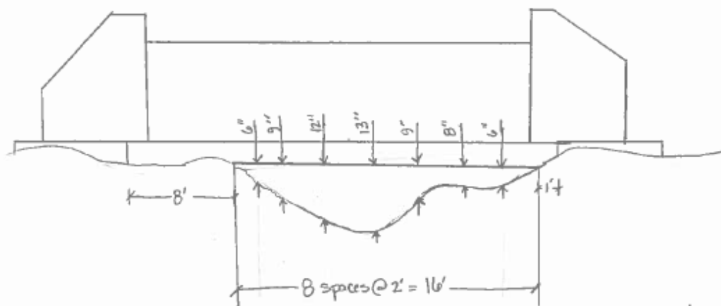
Elevation View
