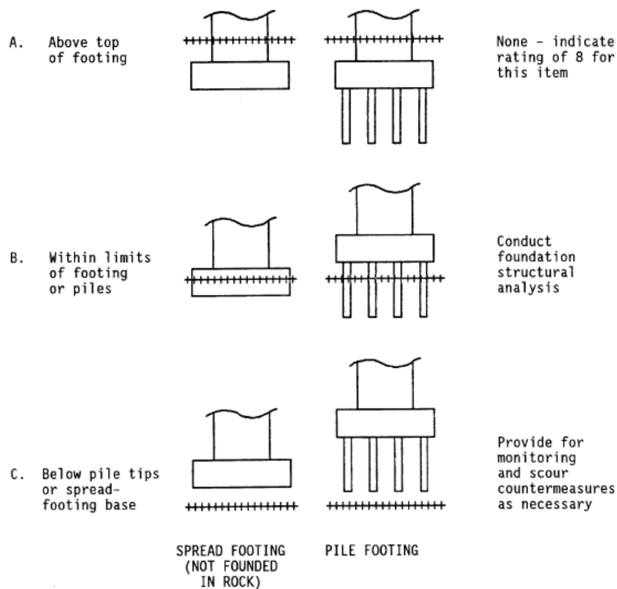
Figure 1: Example of Calculated Scour Depths and Foundations
